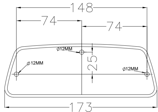
AC-99N Line Drawing
