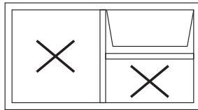
Outward Open Tophung with Bottom & Side Fixed
