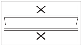
Outward Open Tophung with Top & Bottom Fixed
